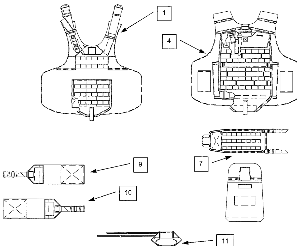
Figure 7. Base Vest Assembly (IOTV Gen II).
